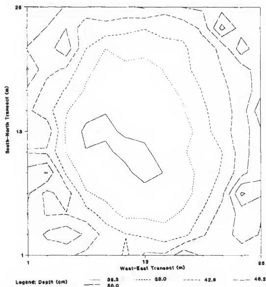
Figure 3. Depth profile of the circular Thalassia testudinum bed at Lassing Park showing mounded bed form.
